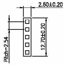
HOUSING
